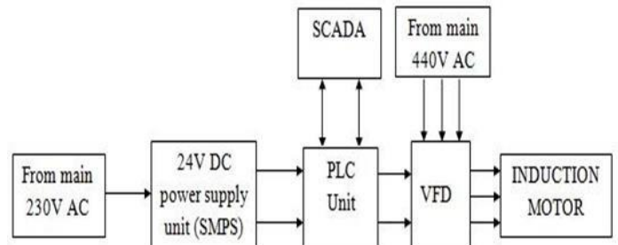
Fig.3 Block Diagram
